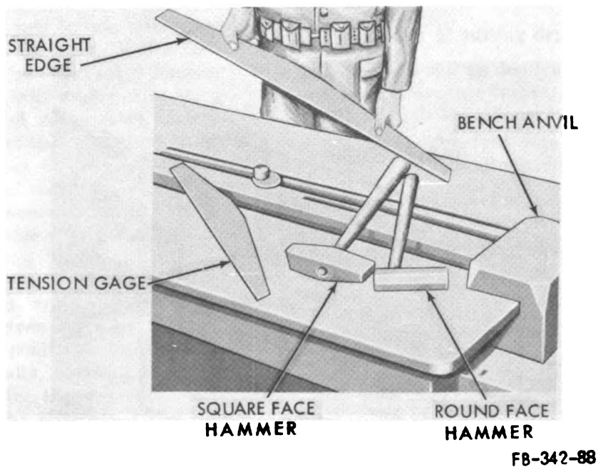
Figure 10-5. Equipment for tensioning saw.
